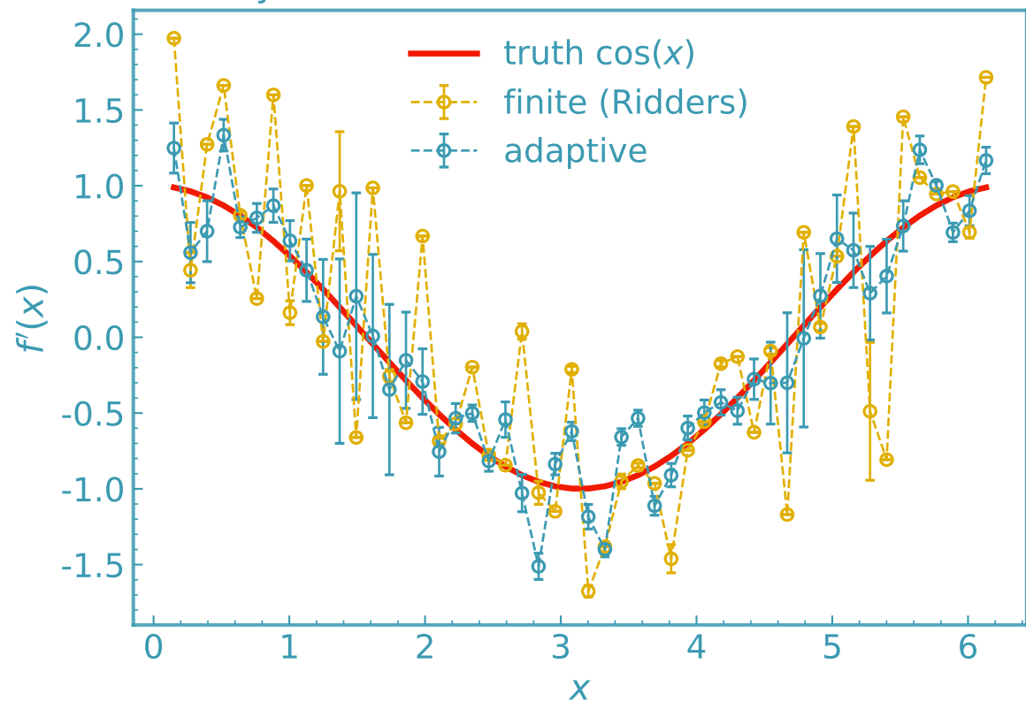
Noisy tabulated derivative estimates vs truth
