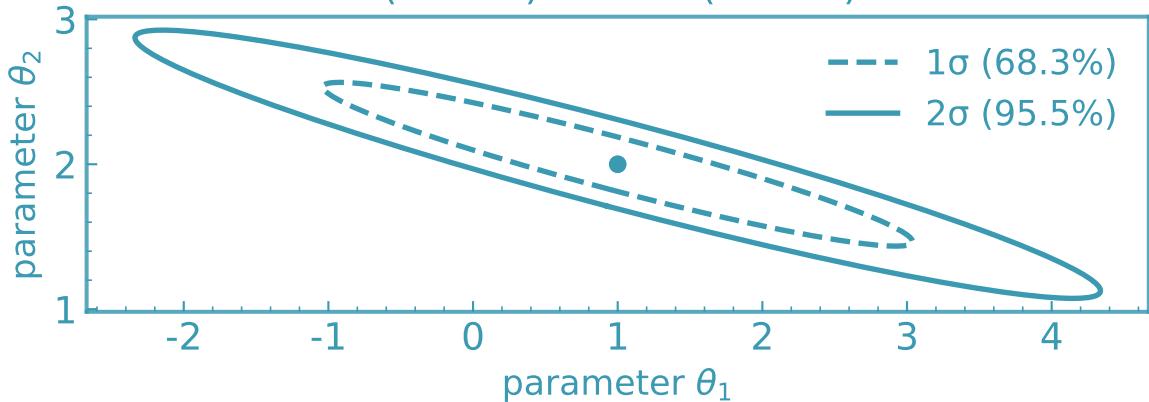
Fisher 1\sigma (68.3%) and 2\sigma (95.5%) contours
