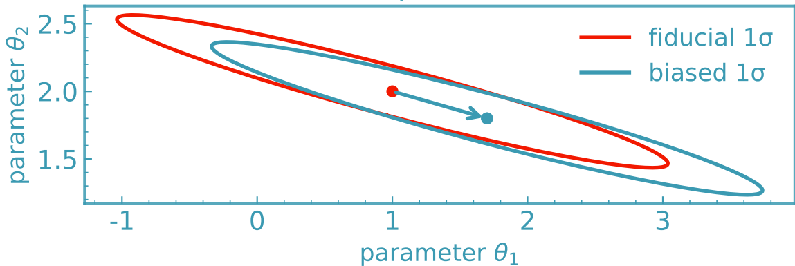
Fisher bias: 1\sigma ellipses (fiducial vs biased)
