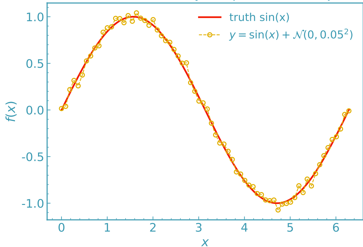
Exact function and noisy samples (Gaussian jitter)
