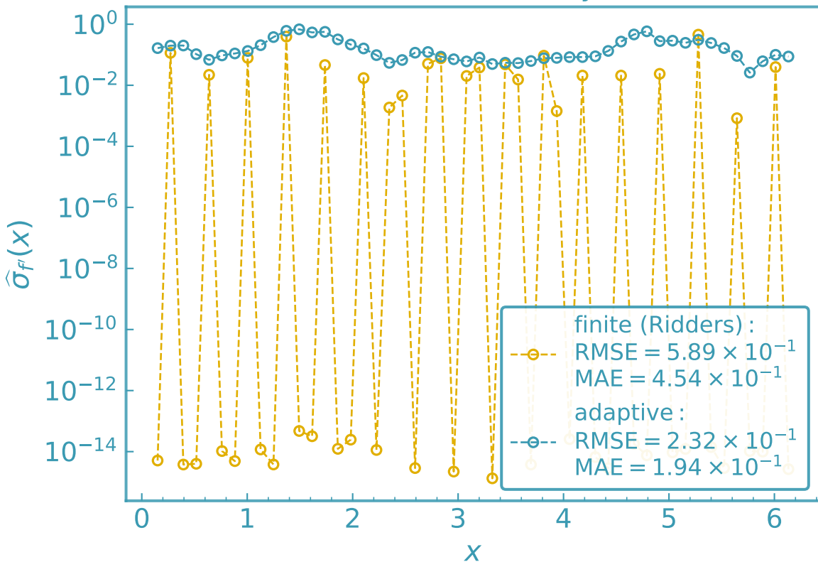
Derivative internal error vs noisy tabulated data
