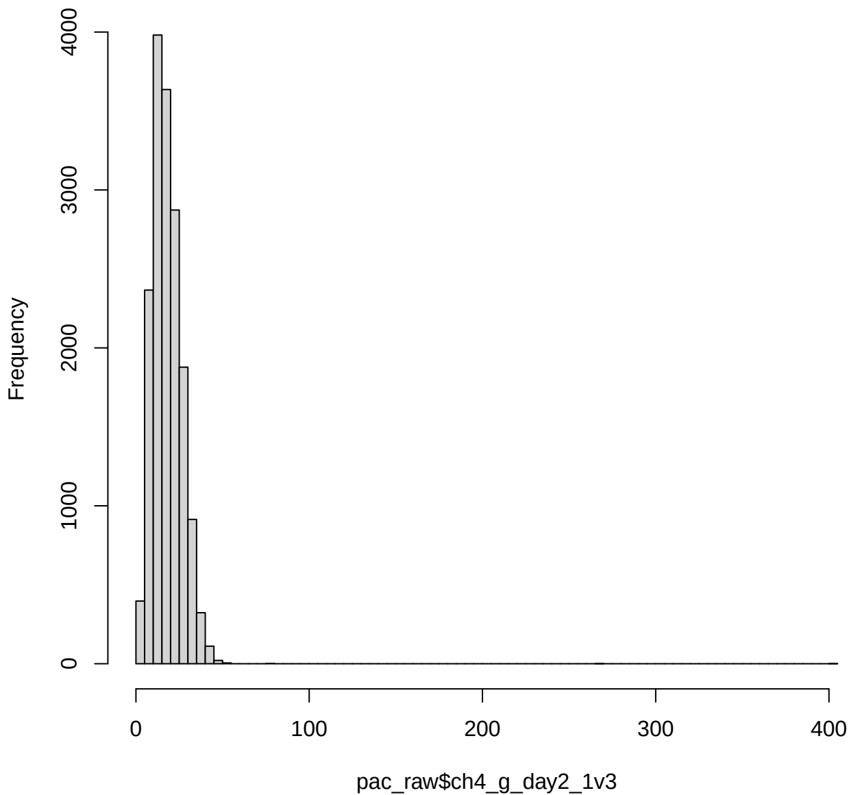
Histogram of pac_raw$ch4_g_day2_1v3
