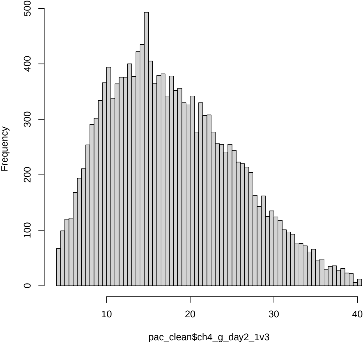
Histogram of pac_clean$ch4_g_day2_1v3
