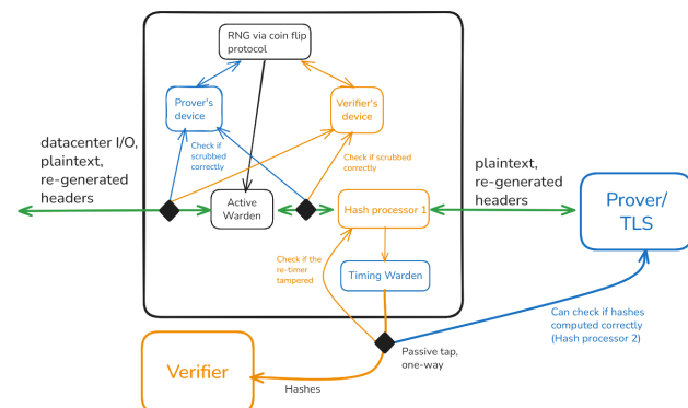
Figure 4. When north-south egress traffic from the datacenter hits the SGD, we first scrub non-reproducible fields with an Active Warden. Where necessary, we use a coin flip protocol as a source of randomness. Traffic leaving the Active Warden is hashed and forwarded. Components drawn in orange represent components that the Verifier relies on to behave correctly, and components drawn in blue represent the same for the Prover.
