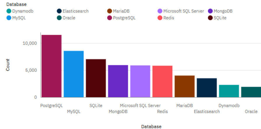
Top 10 DatabaseHaveWorkedWith
