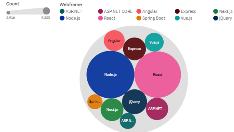
Top 10 WebFrameHaveWorkedWith
