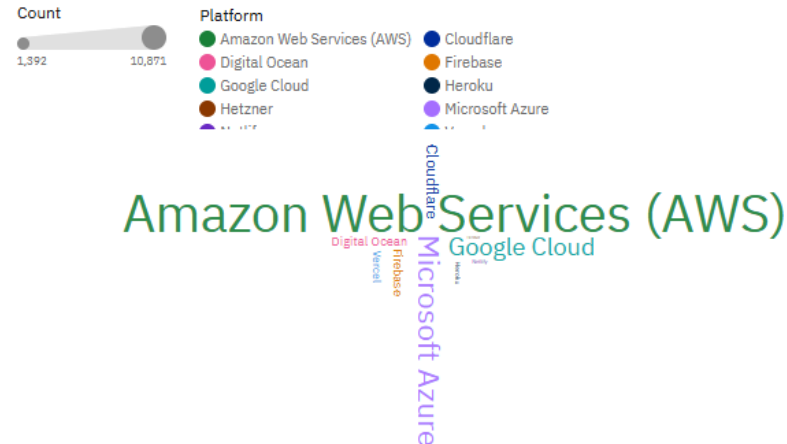
Top 10 PlatformHaveWorkedWith
