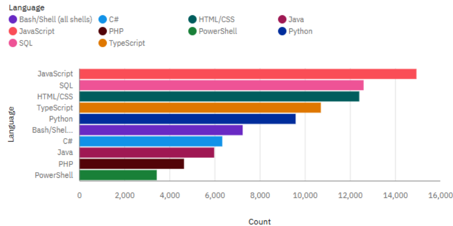
Top 10 LanguageHaveWorkedWith
