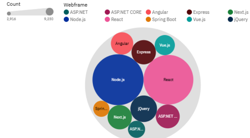
Top 10 WebFrameHaveWorkedWith
