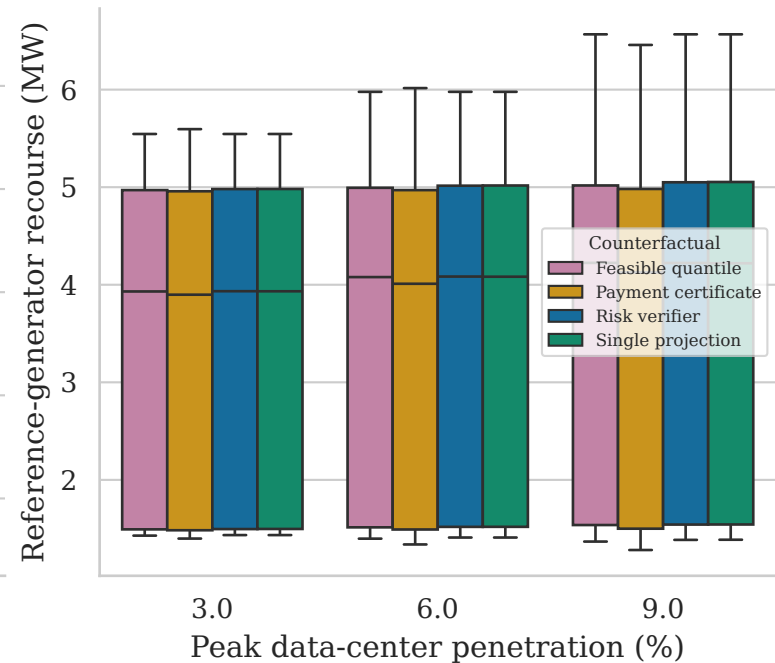
(c) AC-loss balancing recourse
