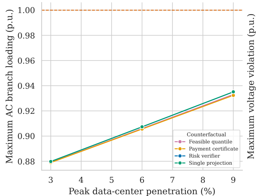
(a) Preventive outage loading envelope
