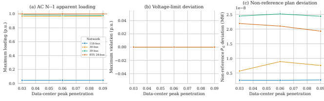
Fig. 4. Cross-network preventive AC N-1 certificate. Each point aggregates the predeclared snapshots and all native-case admissible connected outages; the dashed line in (a) is the unit apparent-power limit.
