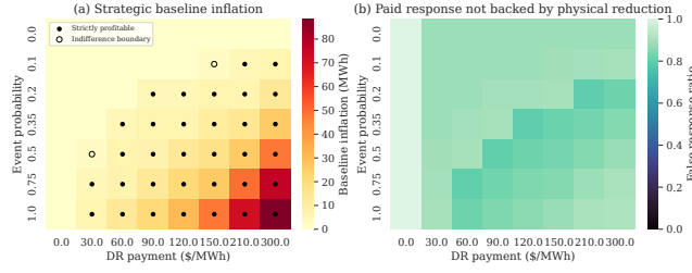
Fig. 3. Experiment 1: exact strategic scheduling across the complete price and call-probability grid. Markers show the independently calculated dual boundary.
