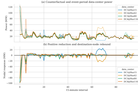
Fig. 5. Experiment 4: predeclared spatial case. Source reduction and destination rebound are evaluated jointly by signed nodal value.
