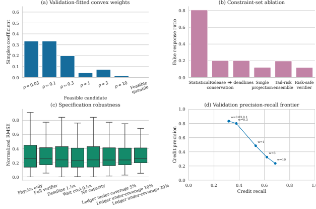
Fig. 4. Experiment 2: validation-fitted projection weights, constraint-set ablation, specification robustness, and the precision-recall frontier. Every point is produced by a globally solved workload program.
