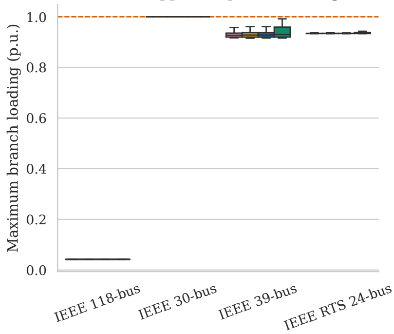
(b) AC apparent-power loading
