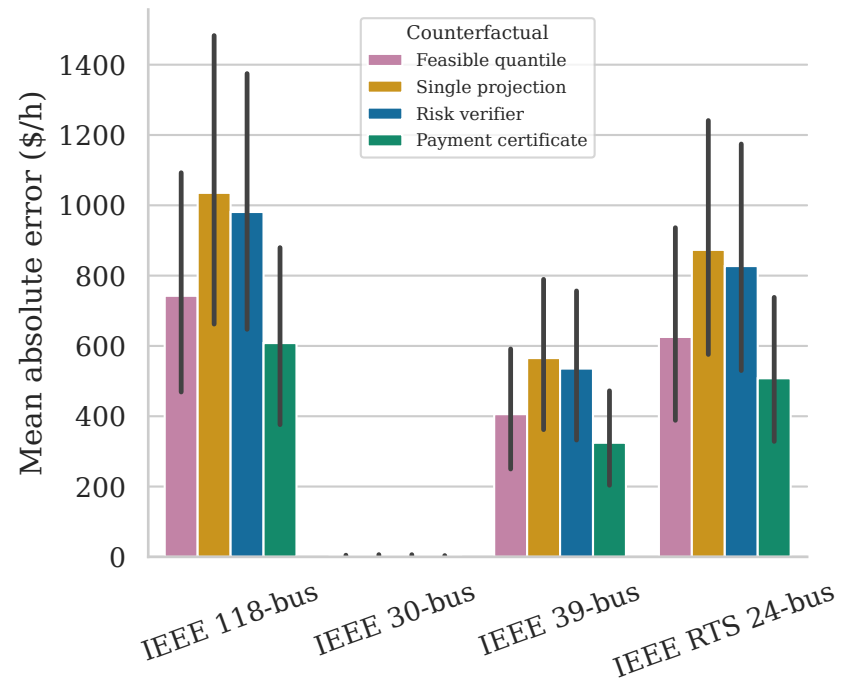
(a) Nonlinear AC value error
