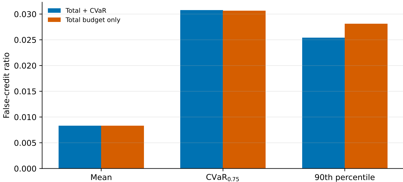
Held-out tail control under the paired risk ablation
