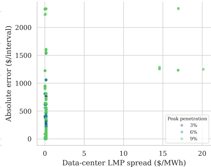
(c) Congestion heterogeneity and error
