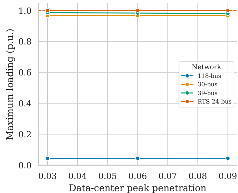
(a) AC N-1 apparent loading
