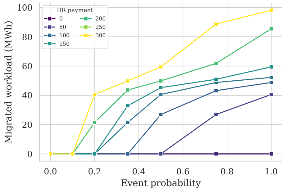
(b) Strategic reference-period migration
