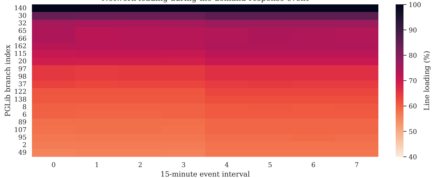
Network loading during the demand-response event
