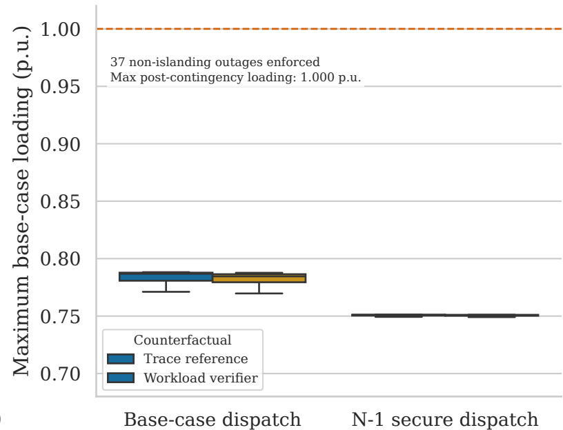
(c) Security-constrained network loading
