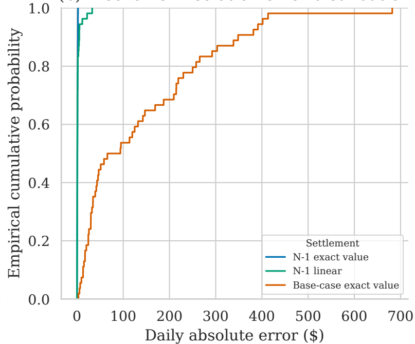
(b) Mechanism-isolation error distribution
