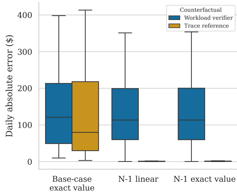
(a) Security-aware payment error
