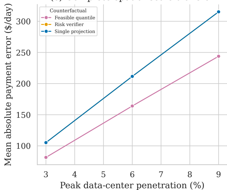
(c) Complete spatial-scale transfer
