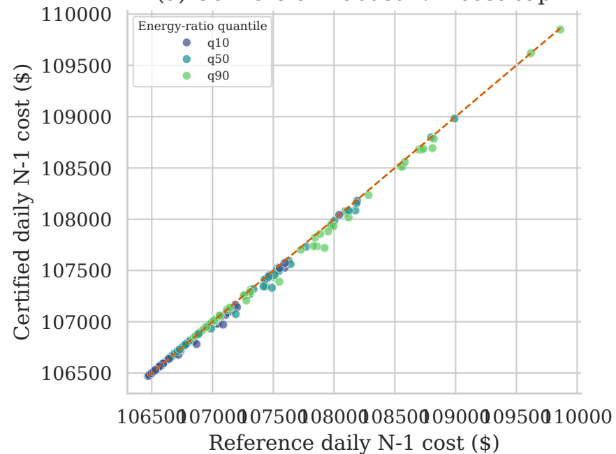
(a) Conversion-robust N-1 cost cap
