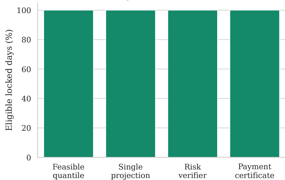
(c) Individually rational contract activation
