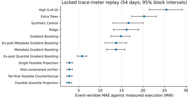
Fig. 3. Independent locked-day trace-meter replay. Points show mean event-window MAE against the measured execution tensor; whiskers are three-day moving-block 95% intervals. The panel is observational and contains no utility-event label.
