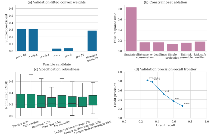
Fig. 4. Validation-fitted projection weights, constraint-set ablation, specification robustness, and the precision-recall frontier. Every point is produced by a globally solved workload program.
