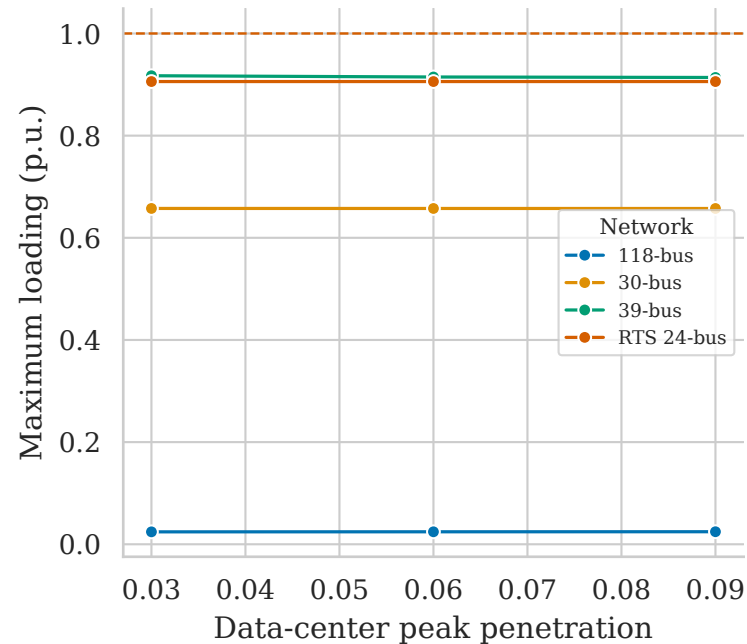
(a) AC N-1 apparent loading
