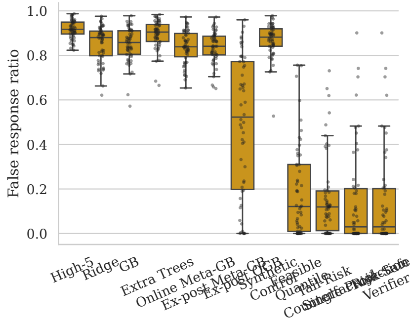
(b) False response exposure
