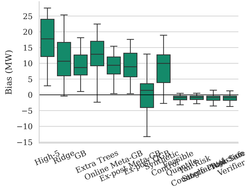
(c) Event-window bias
