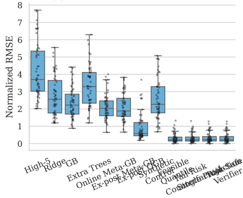
(a) Counterfactual baseline error
