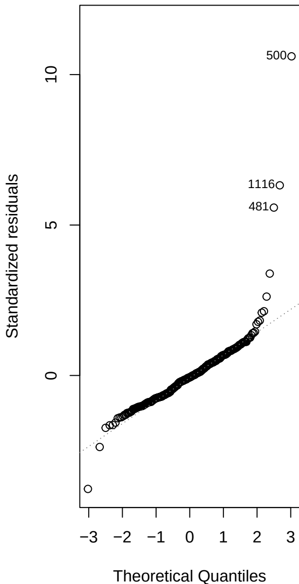
Q-Q Residuals
