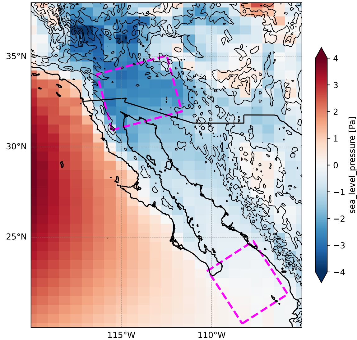
SLP anomaly rel. to global mean
