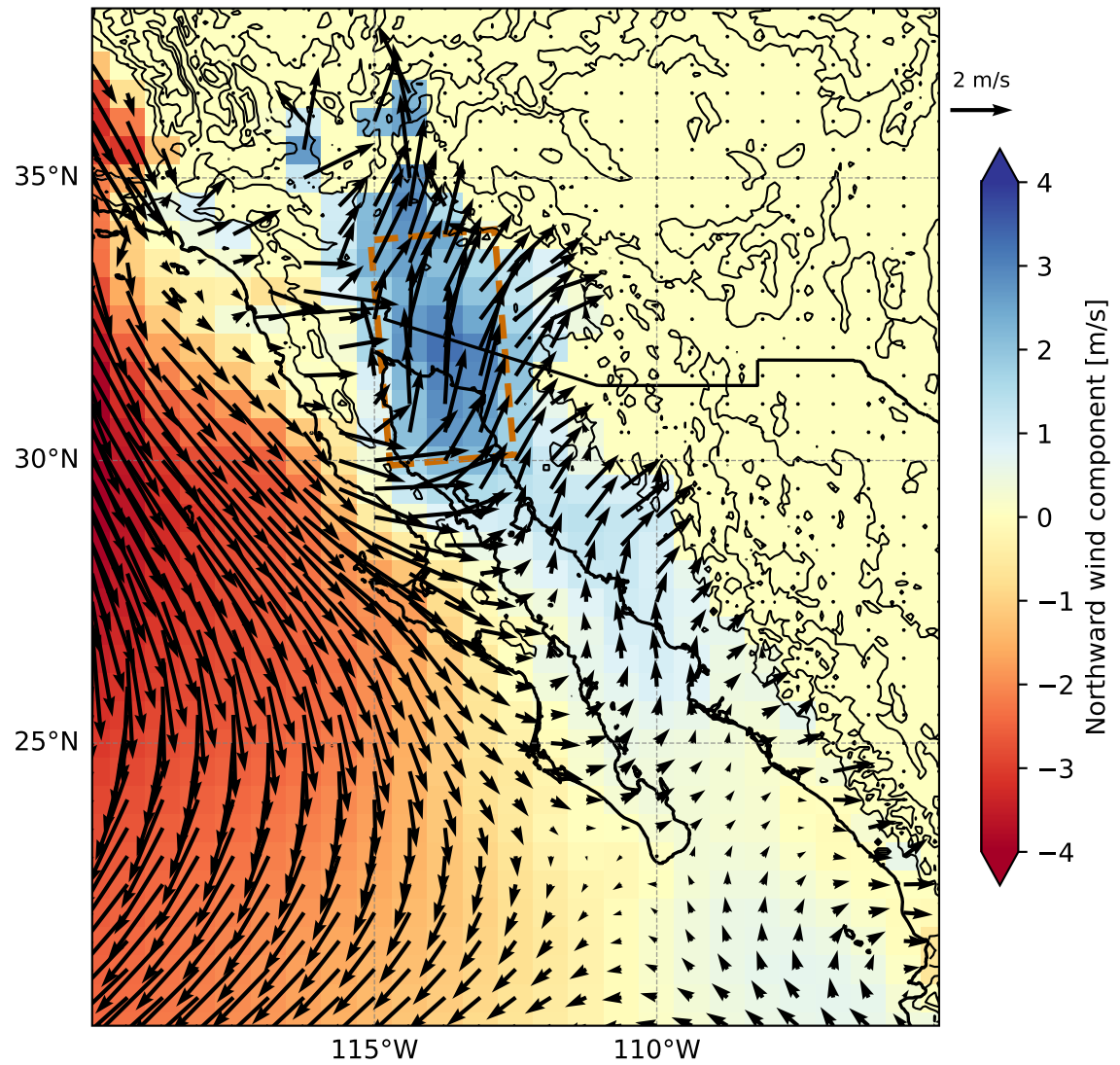
925 hPa wind
