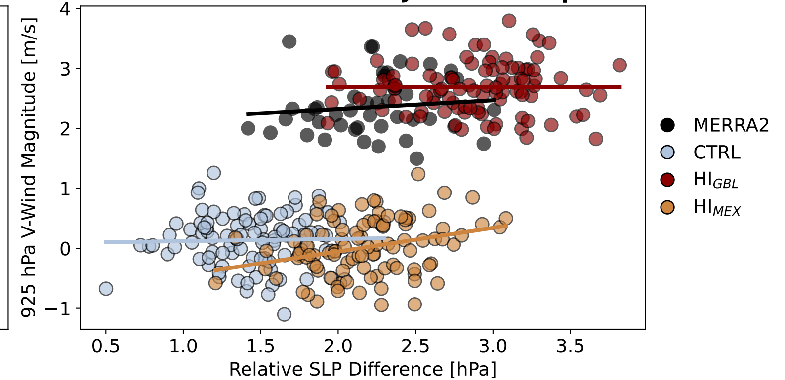
F SLP Gradient-GoCLLJ Relationship
