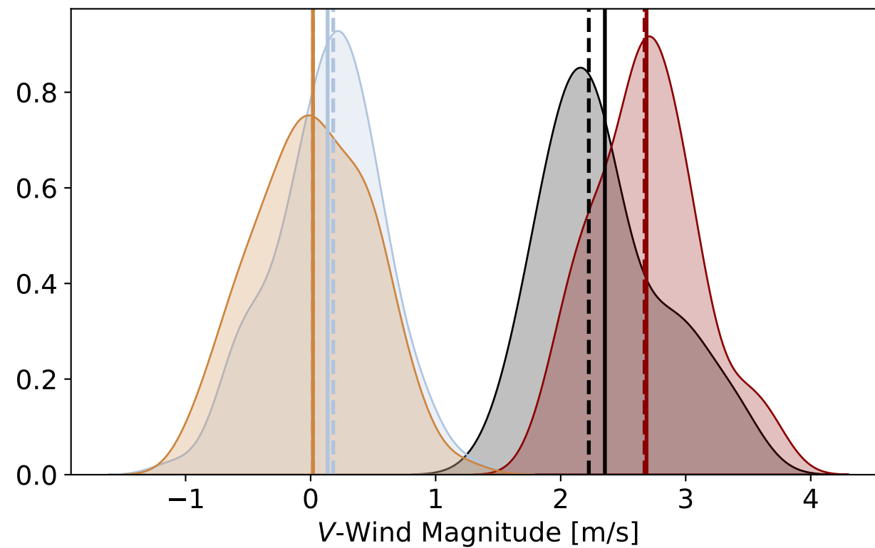
E 925 hPa Meridional Wind
