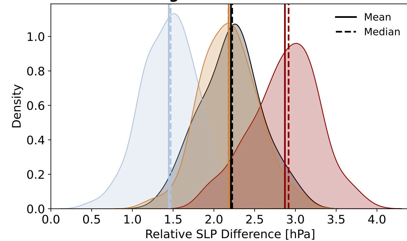
D Along-Gulf SLP Gradient
