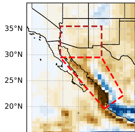
High-Res. MME
