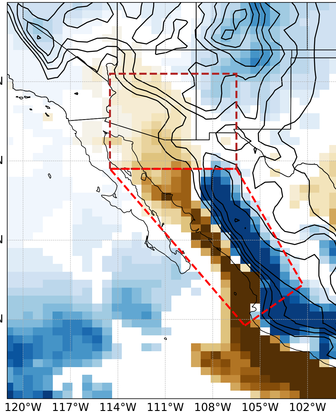
A CTRL-IMERG
