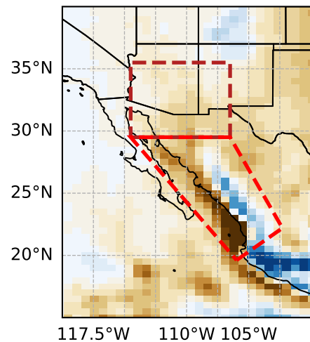
High-Res. MME
