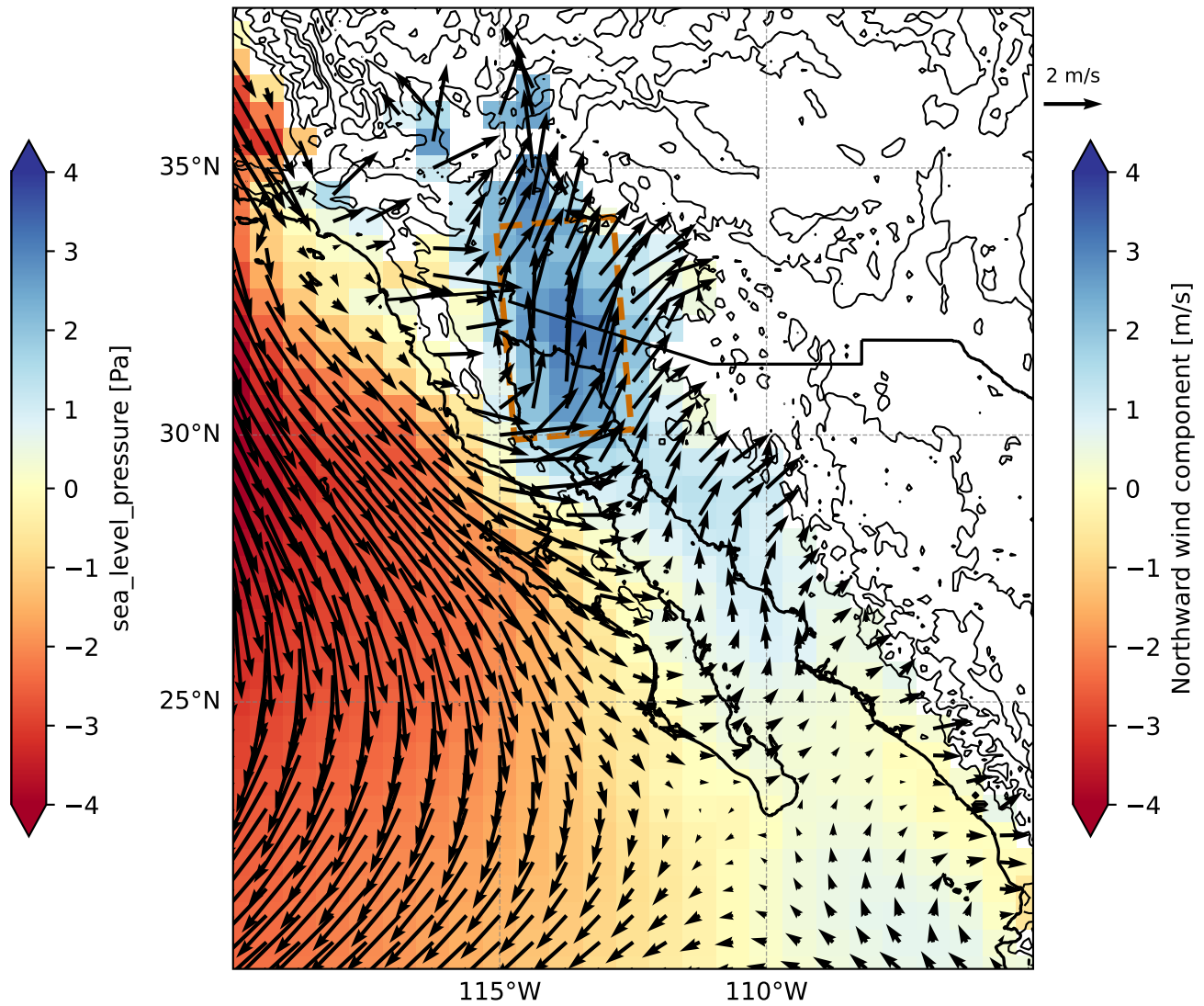
925 hPa wind
