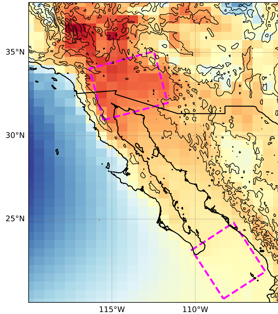
SLP anomaly rel. to global mean
