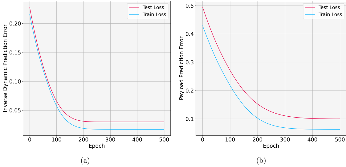
Figure 6: Transfer learning process, where the data split ratio is 8:2, and all data have been normalized. (a) IDM (b) PE.
