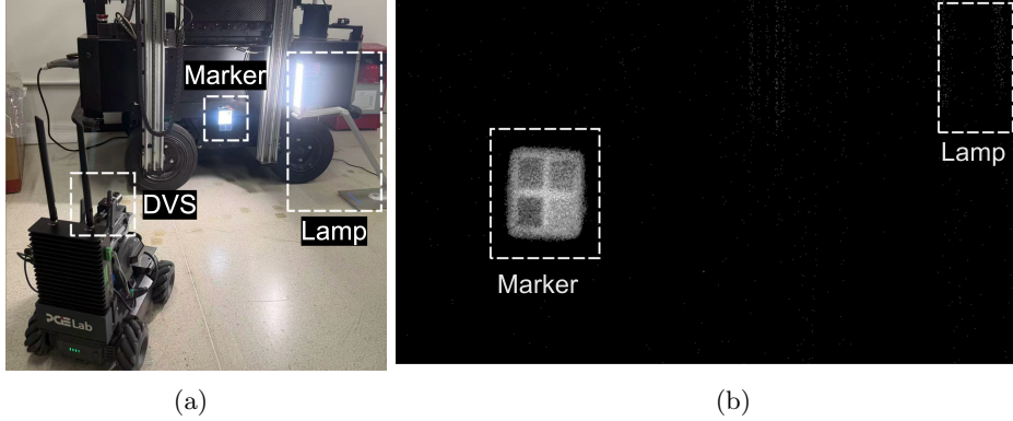
Figure 3: (a) Scenario with a lamp as ambient flicker. (b) Marker perceived by DVS with a duration of 2ms with ambient flicker aside.
