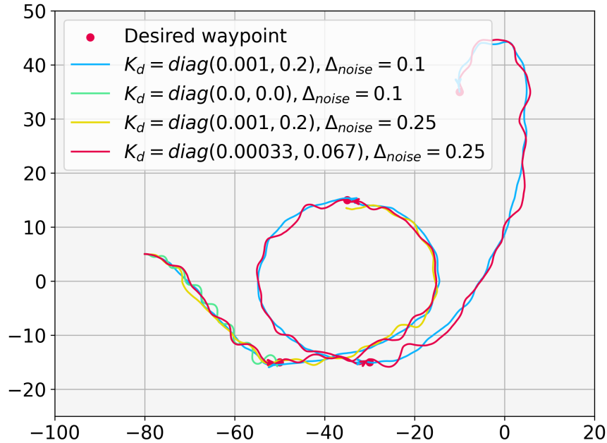
Figure 5: Performance comparison of different \mathbf{K}_d with different observation noise \Delta_{\text{noise}} .
