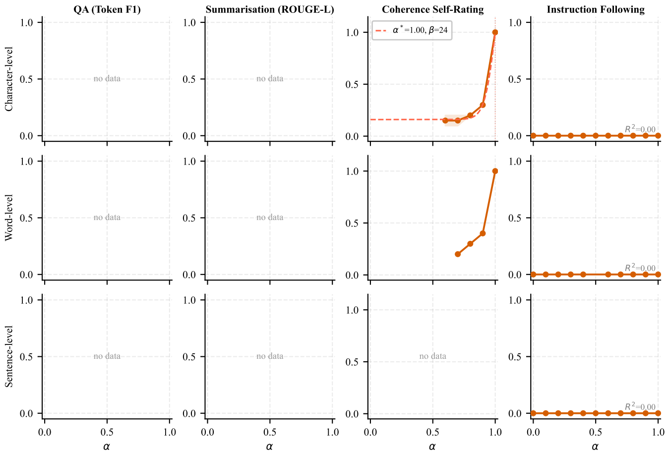
Figure 3: Claude Sonnet 4.5 — All Tasks × Granularities (dashed = sigmoid fit, dotted vertical = \alpha^* )
