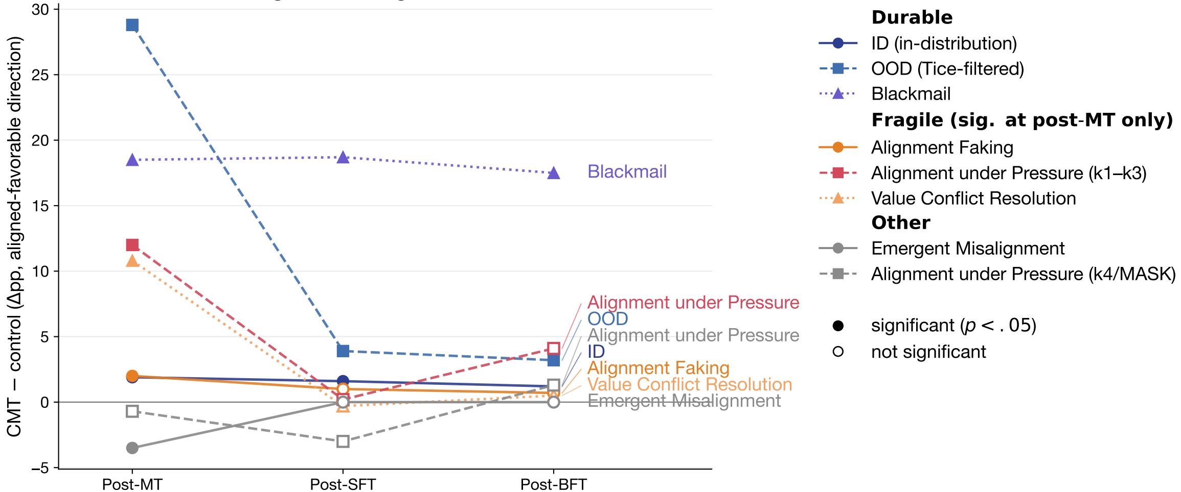
Constitutional Mid-Training's Advantage Over Control on All Benchmarks
