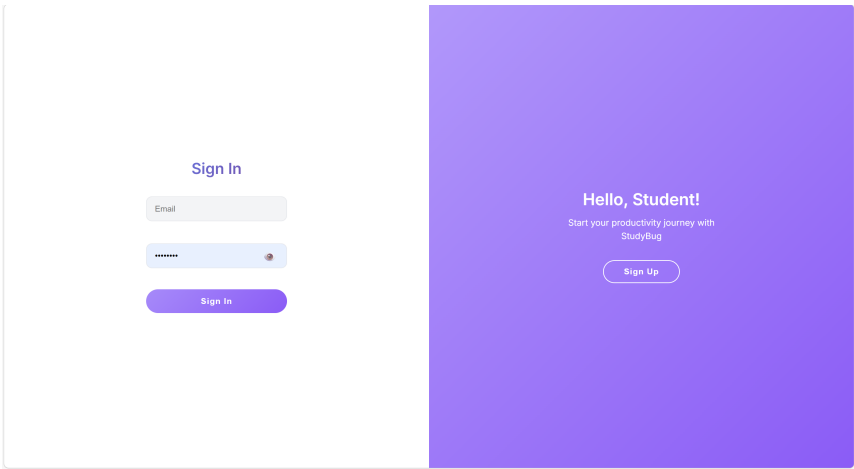
Figure 8.2: Login Interface
