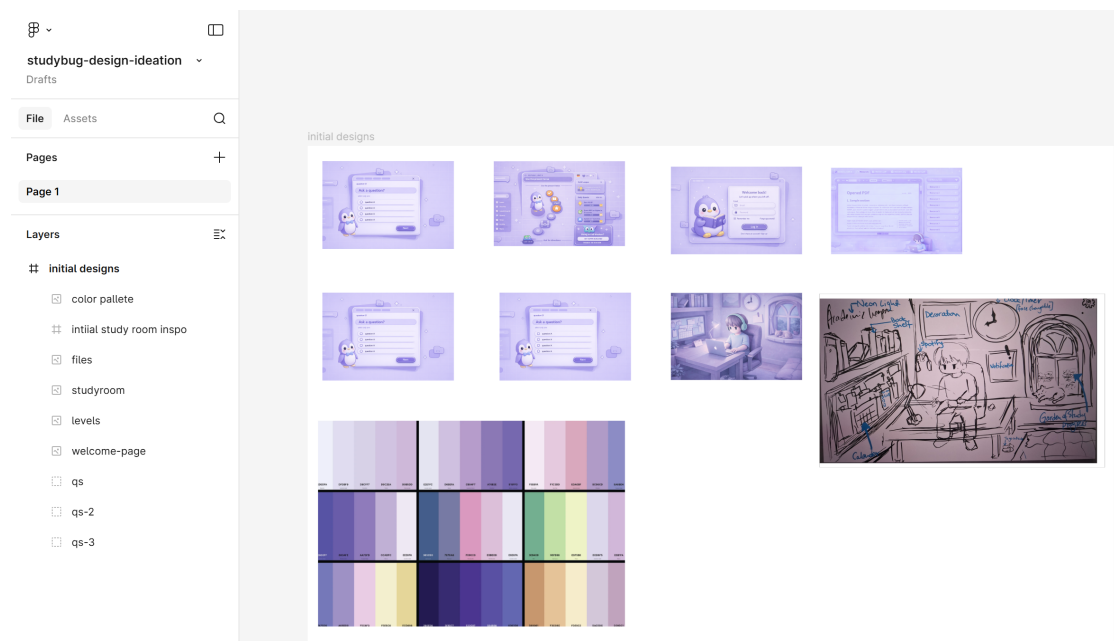
Figure 4.3: Figma Workflow
