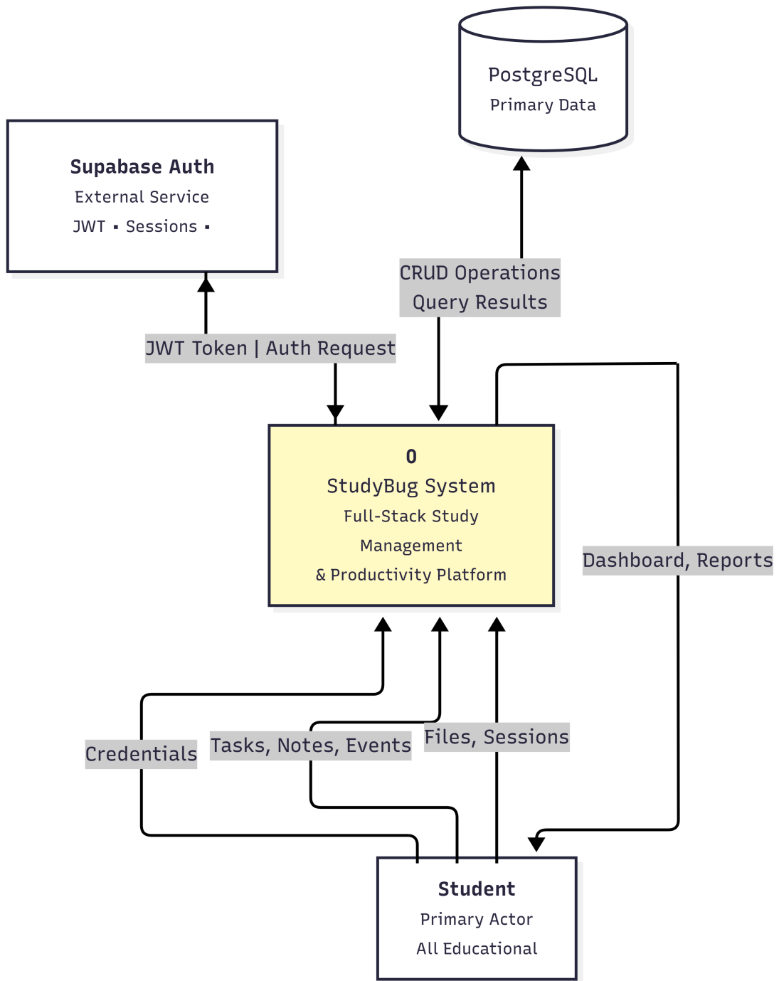
Figure 6.2: Context Diagram of StudyBug
