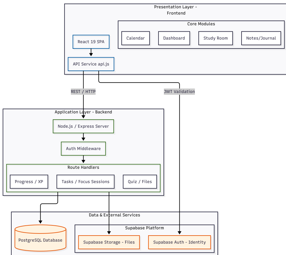
Figure 6.5: System Block Diagram of StudyBug
