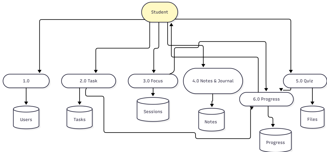
Figure 6.3: Data Flow Diagram of StudyBug
