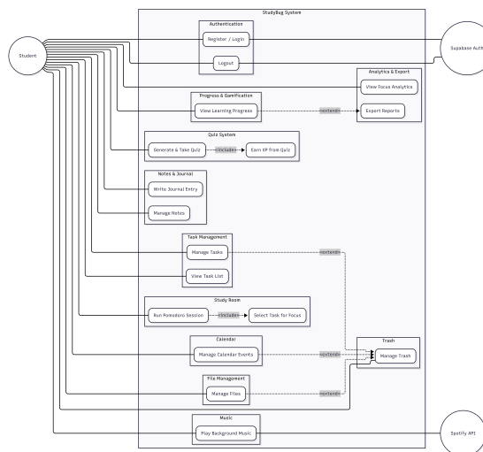
Figure 6.1: Use Case Diagram of StudyBug
