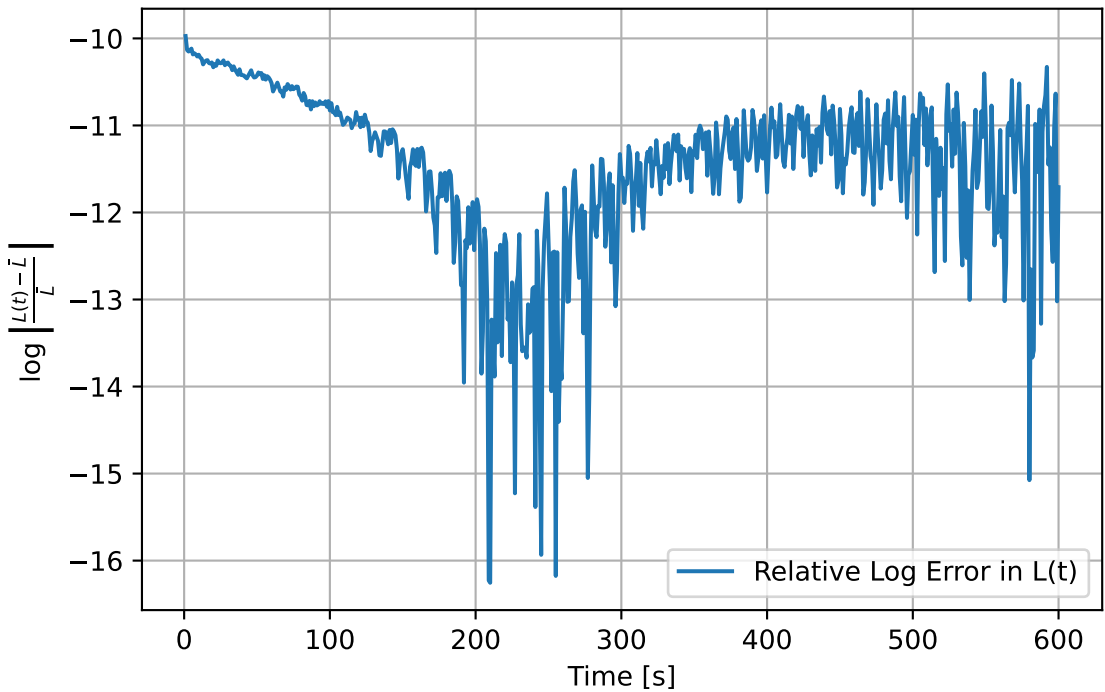
Relative Log Error of Angular Momentum over Time
