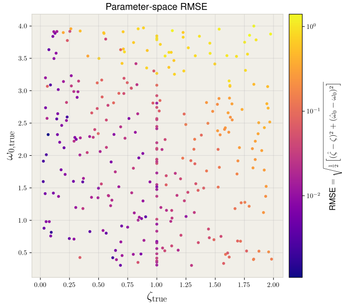
Figure 2.25: Parameter space of 304 true (\zeta, \omega_0) pairs and the RMSE compared to the predicted values.
