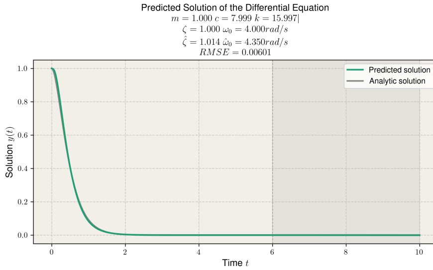
Figure 2.20: Predicted solution and parameters for a critically damped harmonic oscillator with randomised parameters.
