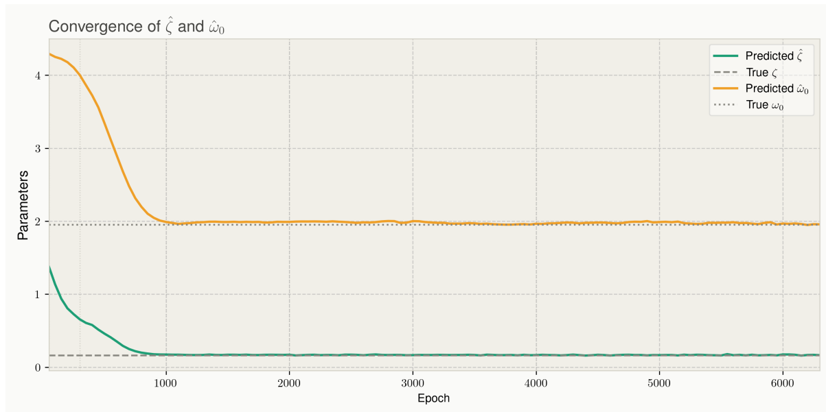
Figure 2.16: Parameter convergence to true values for an underdamped harmonic oscillator with randomised parameters.
