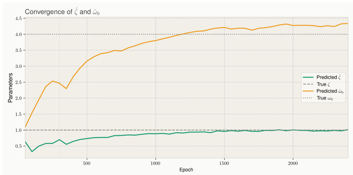
Figure 2.14: Parameter convergence to true values for a critically damped harmonic oscillator with randomised parameters.
