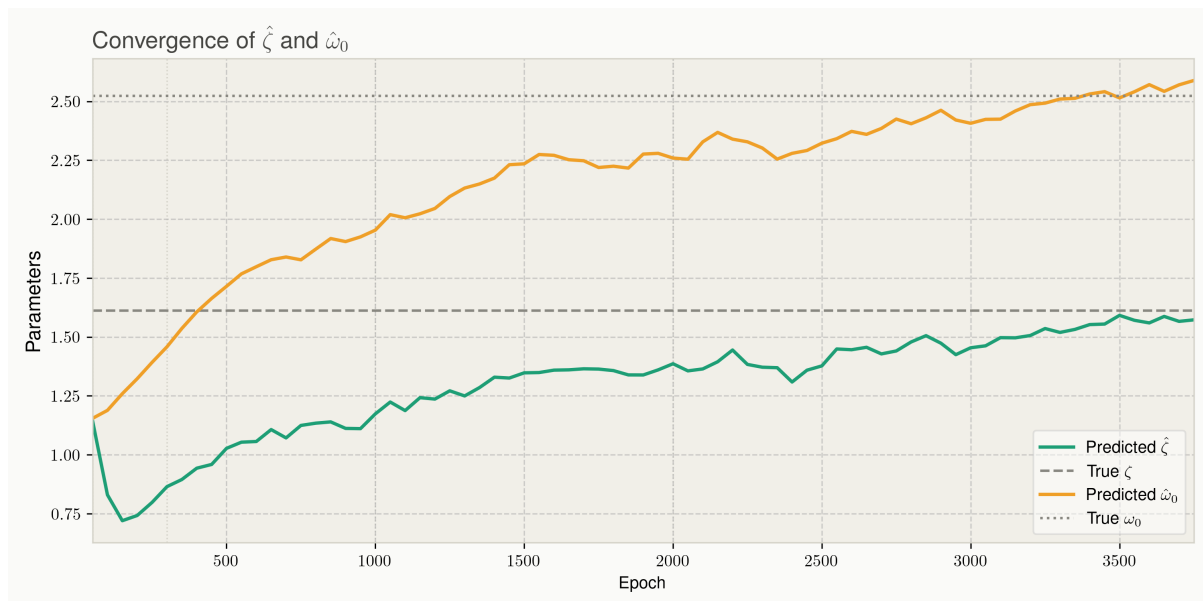
Figure 2.12: Parameter convergence to true values for an overdamped harmonic oscillator with randomised parameters.
