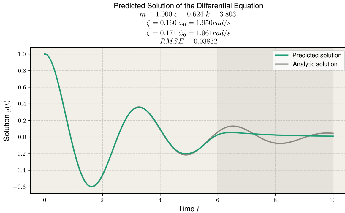
Figure 2.15: Predicted solution and parameters for an underdamped harmonic oscillator with randomised parameters.
