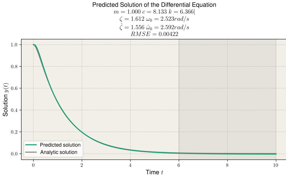
Figure 2.11: Predicted solution and parameters for an overdamped harmonic oscillator with randomised parameters.
