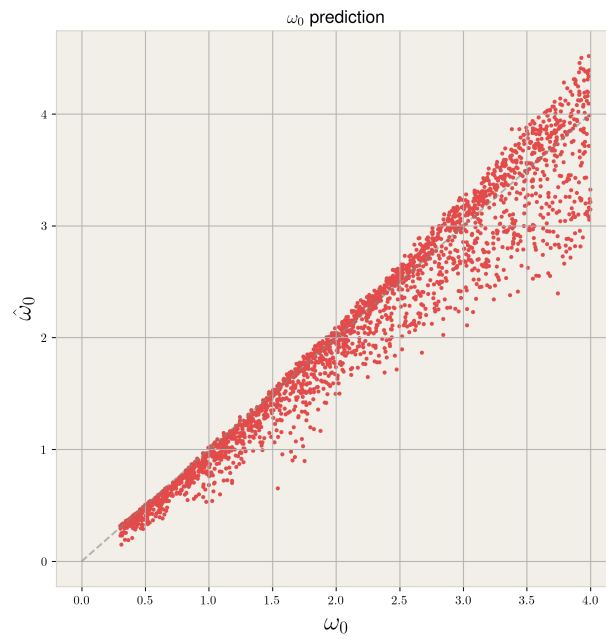
Figure 2.18: Scatter plot of 2402 true and predicted \omega_0 pairs for the damped harmonic oscillator.
