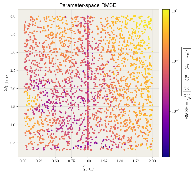
Figure 2.19: Parameter space of 2402 true (\zeta, \omega_0) pairs and the RMSE compared to the predicted values..
