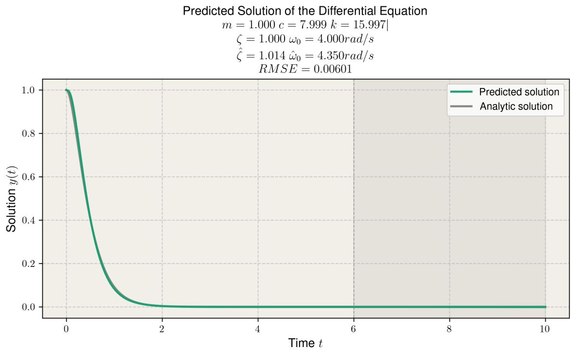
Figure 2.13: Predicted solution and parameters for a critically damped harmonic oscillator with randomised parameters.
