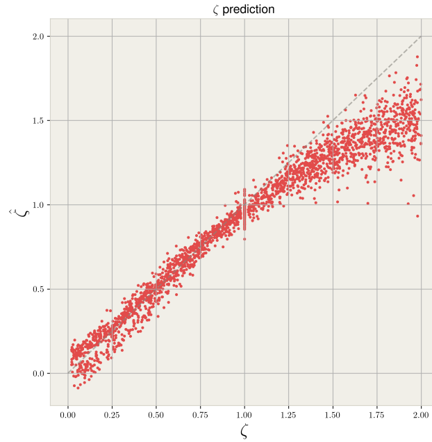
Figure 2.17: Scatter plot of 2402 true and predicted \zeta pairs for the damped harmonic oscillator.
