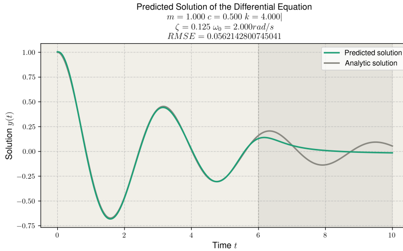
Figure 2.15: Predicted solution with standard hyperparameters shown in Table 2.1
