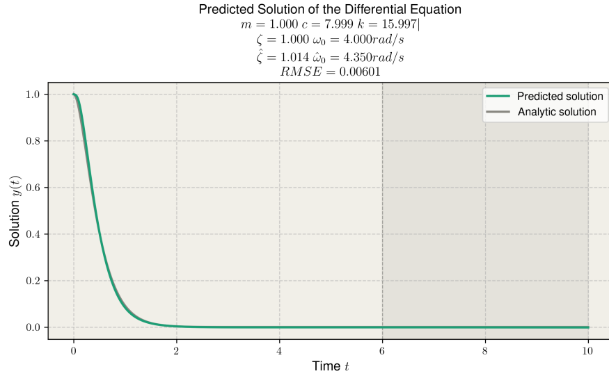
Figure 2.24: Predicted solution and parameters for a critically damped harmonic oscillator with randomised parameters.
