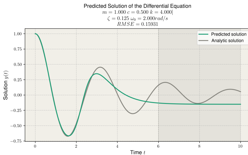
Figure 2.12: Predicted solution from a model with a very low complexity.
