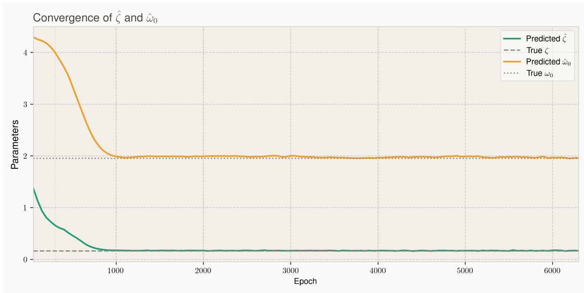
Figure 2.23: Parameter convergence to true values for an underdamped harmonic oscillator with randomised parameters.
