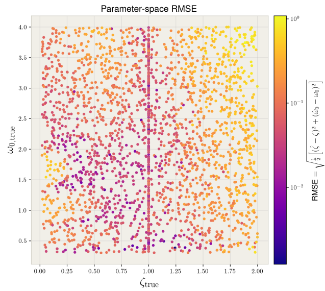
Figure 2.26: Parameter space of 2402 true (\zeta, \omega_0) pairs and the RMSE compared to the predicted values..
