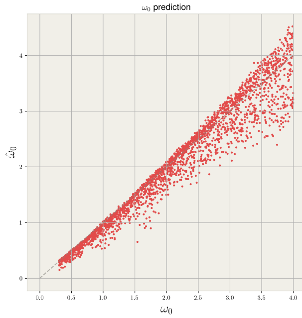
Figure 2.25: Scatter plot of 2402 true and predicted \omega_0 pairs for the damped harmonic oscillator.
