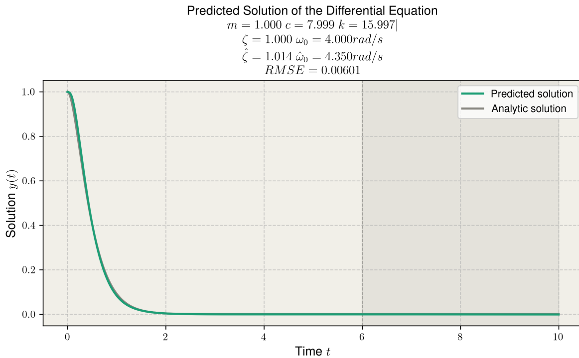
Figure 2.20: Predicted solution and parameters for a critically damped harmonic oscillator with randomised parameters.
