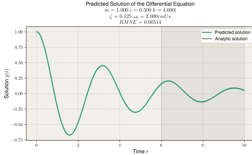
Figure 2.17: Predicted solution with \lambda_{phys} = 100 and no noisy observation points for training.
