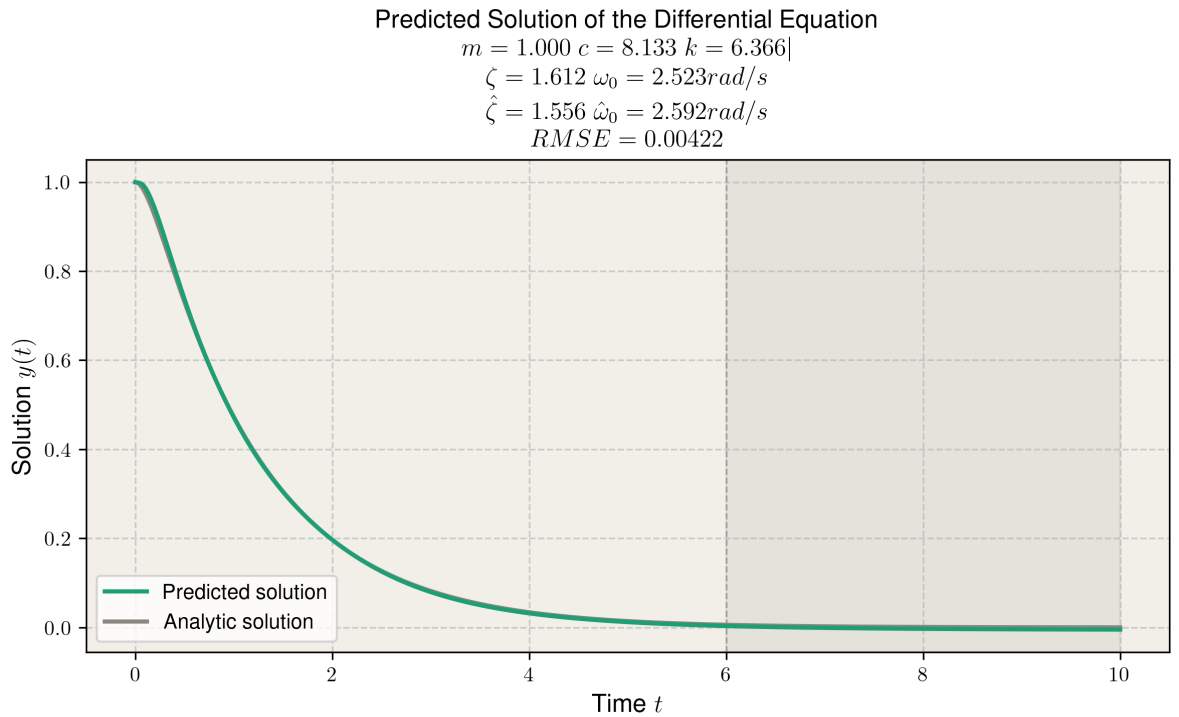
Figure 2.18: Predicted solution and parameters for an overdamped harmonic oscillator with randomised parameters.
