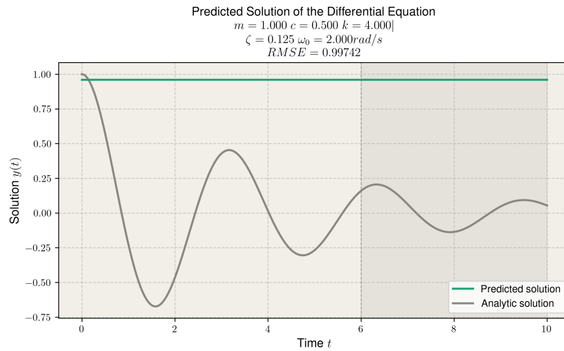
Figure 2.13: Predicted solution with lr = 0.05 .
