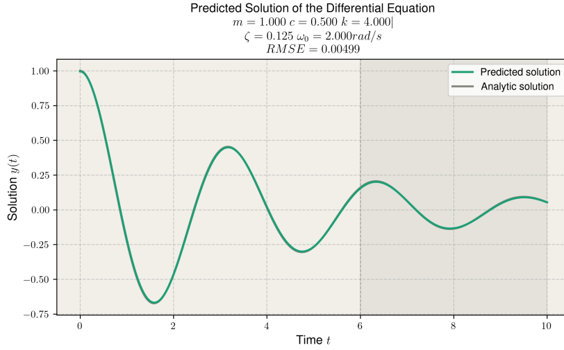
Figure 2.15: Predicted solution with \lambda_{phys} = 100 .
