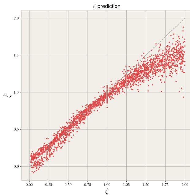
Figure 2.24: Scatter plot of 2402 true and predicted \zeta pairs for the damped harmonic oscillator.
