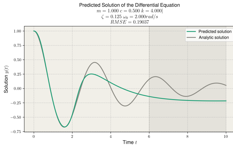
Figure 2.14: Predicted solution with lr = 0.05 .
