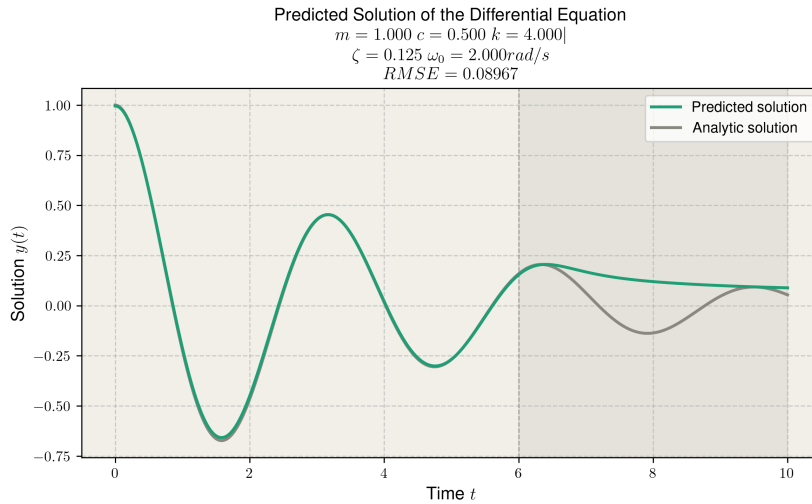
Figure 2.16: Predicted solution with \lambda_{phys} = 100 and no collocation points in the extrapolated domain.
