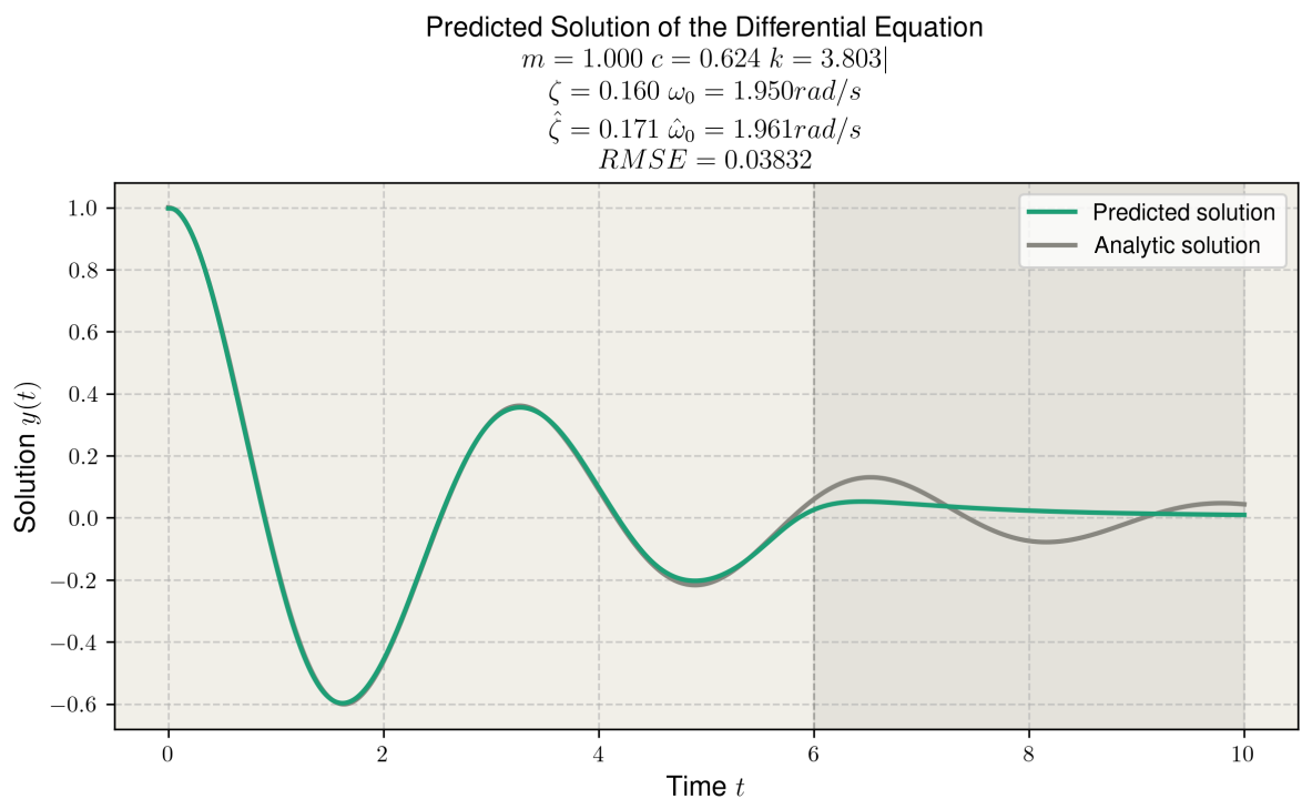
Figure 2.22: Predicted solution and parameters for an underdamped harmonic oscillator with randomised parameters.
