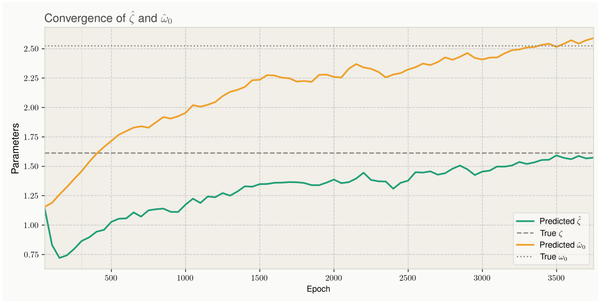
Figure 2.19: Parameter convergence to true values for an overdamped harmonic oscillator with randomised parameters.
