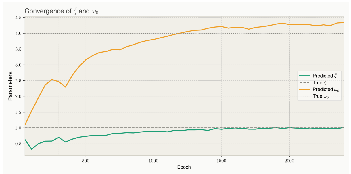
Figure 2.21: Parameter convergence to true values for a critically damped harmonic oscillator with randomised parameters.
