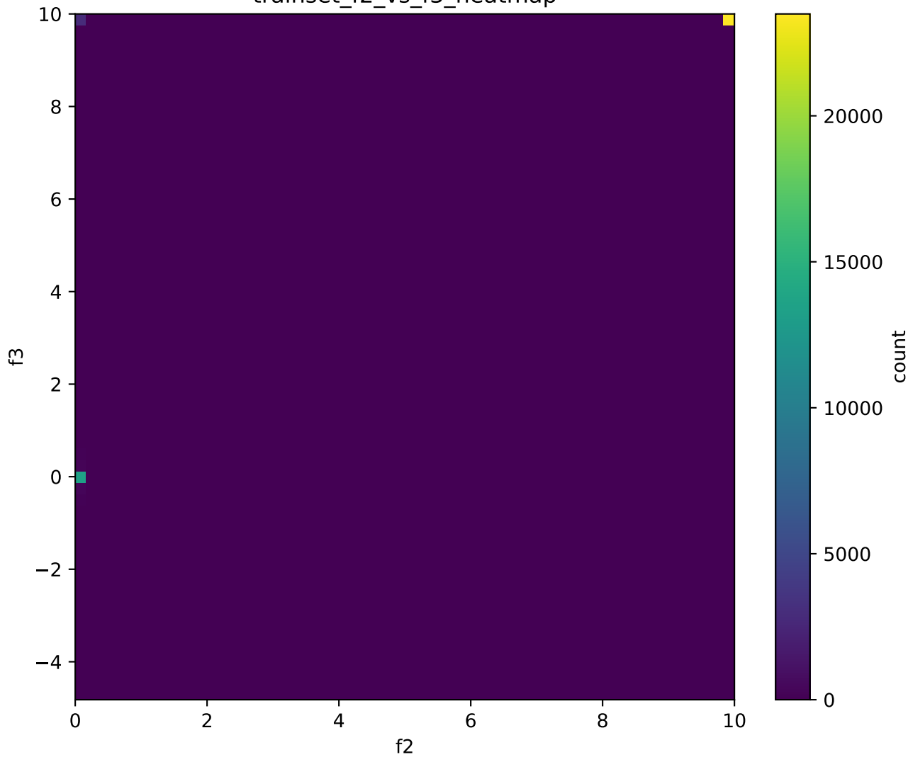
trainset_f2_vs_f3_heatmap
