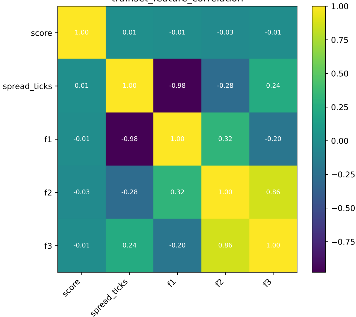
trainset_feature_correlation
