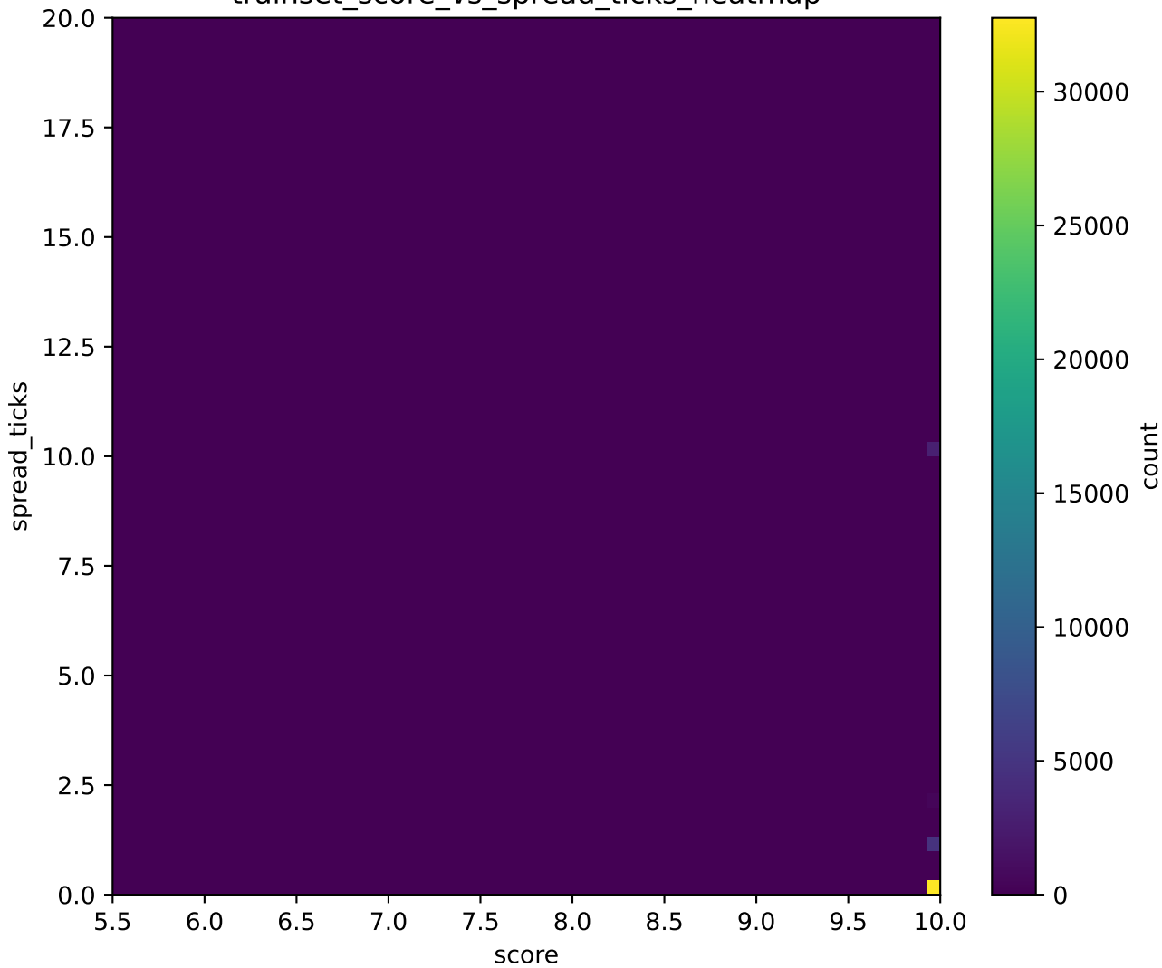
trainset_score_vs_spread_ticks_heatmap
