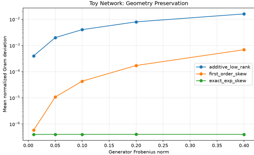
Figure 2(a). Toy network geometry preservation. Mean normalized Gram deviation \overline{\Delta}_G for additive low-rank, first-order skew, and exact exponential skew updates applied to the first-layer weight matrix of a pretrained MNIST MLP, as a function of generator Frobenius norm.
