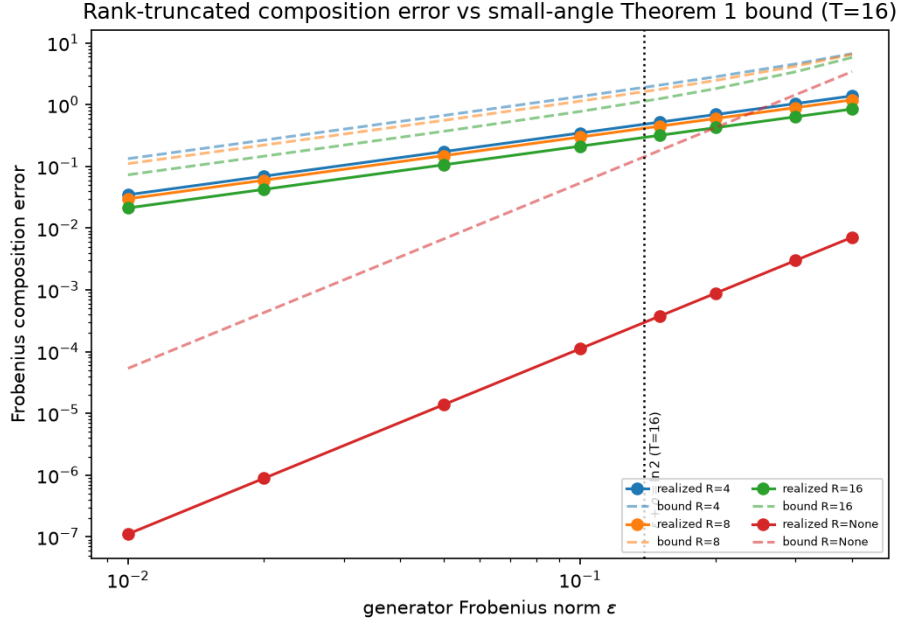
Figure 1(d). Measured composition error of rank-truncated BCH accumulation (solid) against the two-term Theorem 1 bound in its small-angle L = 1 form (dashed; running- \rho BCH remainder plus measured Eckart-Young tail), versus generator Frobenius norm and truncation rank R in \mathfrak{so}(128) at T = 16 . The dotted vertical line marks where the accumulated history leaves Theorem 1’s radius, \varepsilon + \rho = \ln 2 ( \varepsilon \approx 0.14 at T = 16 ): left of it the bound is guaranteed, right of it it is reported as an empirical envelope.
