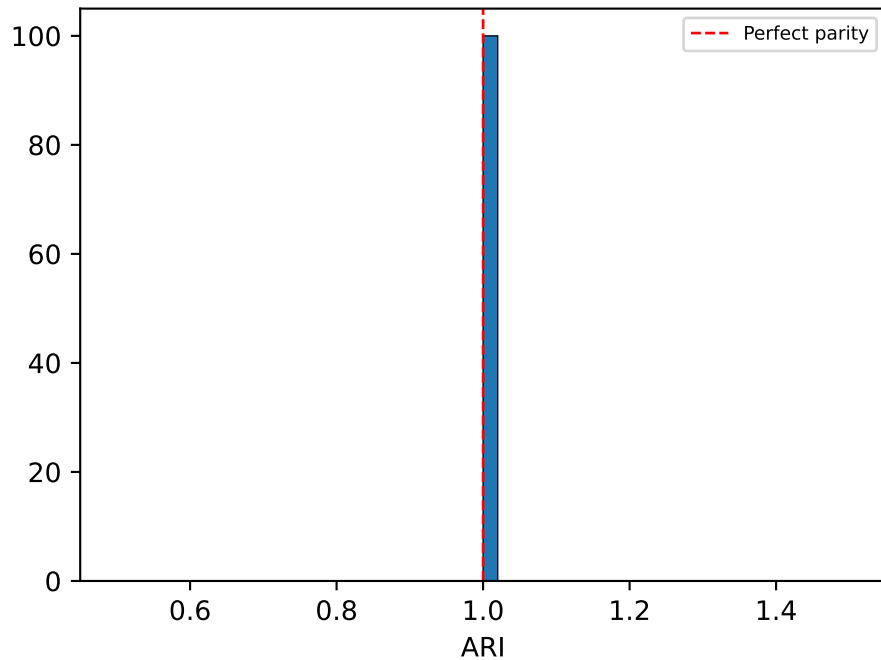
ARI Distribution
