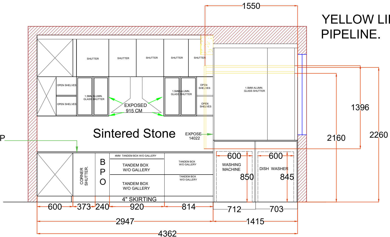
KITCHEN GAS PIPELINE PROPOSE
