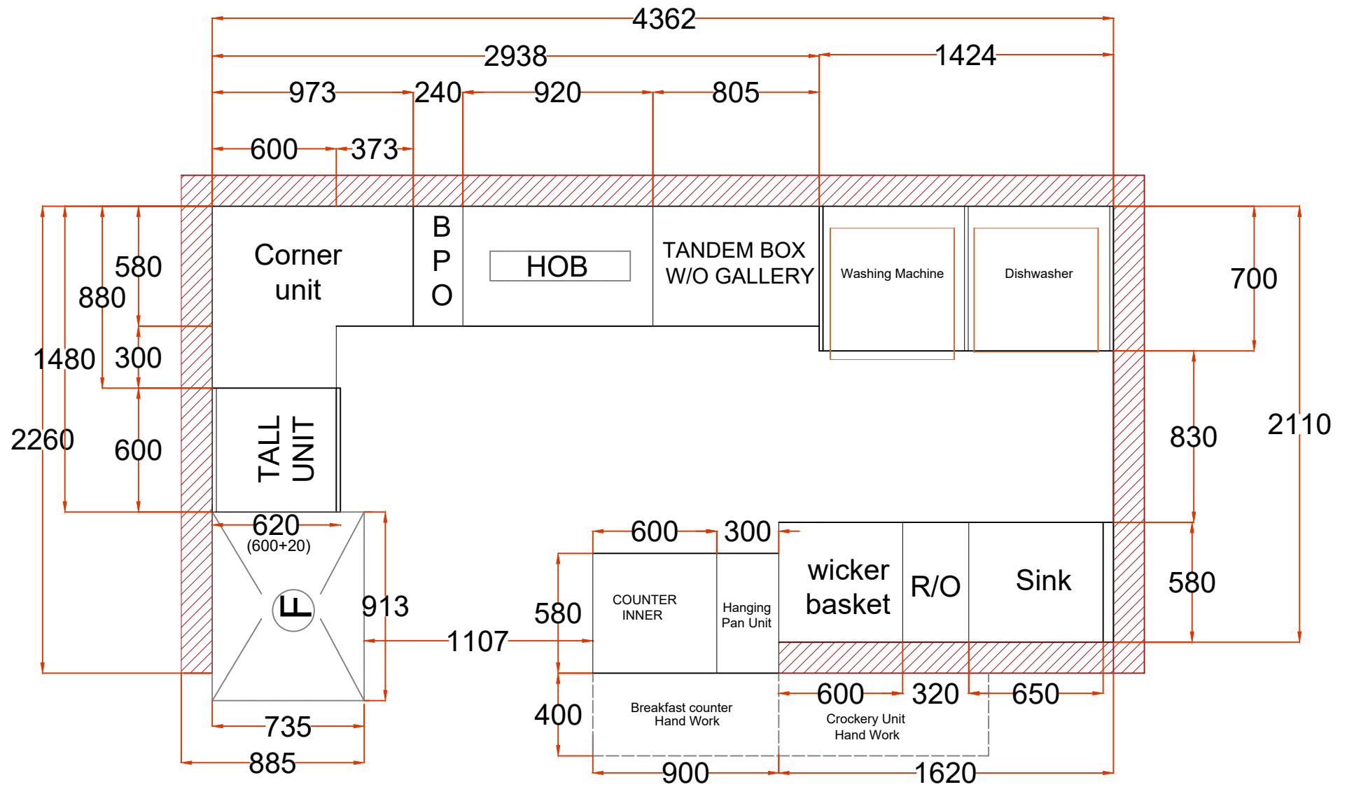
KITCHEN BELOW UNIT PLAN
