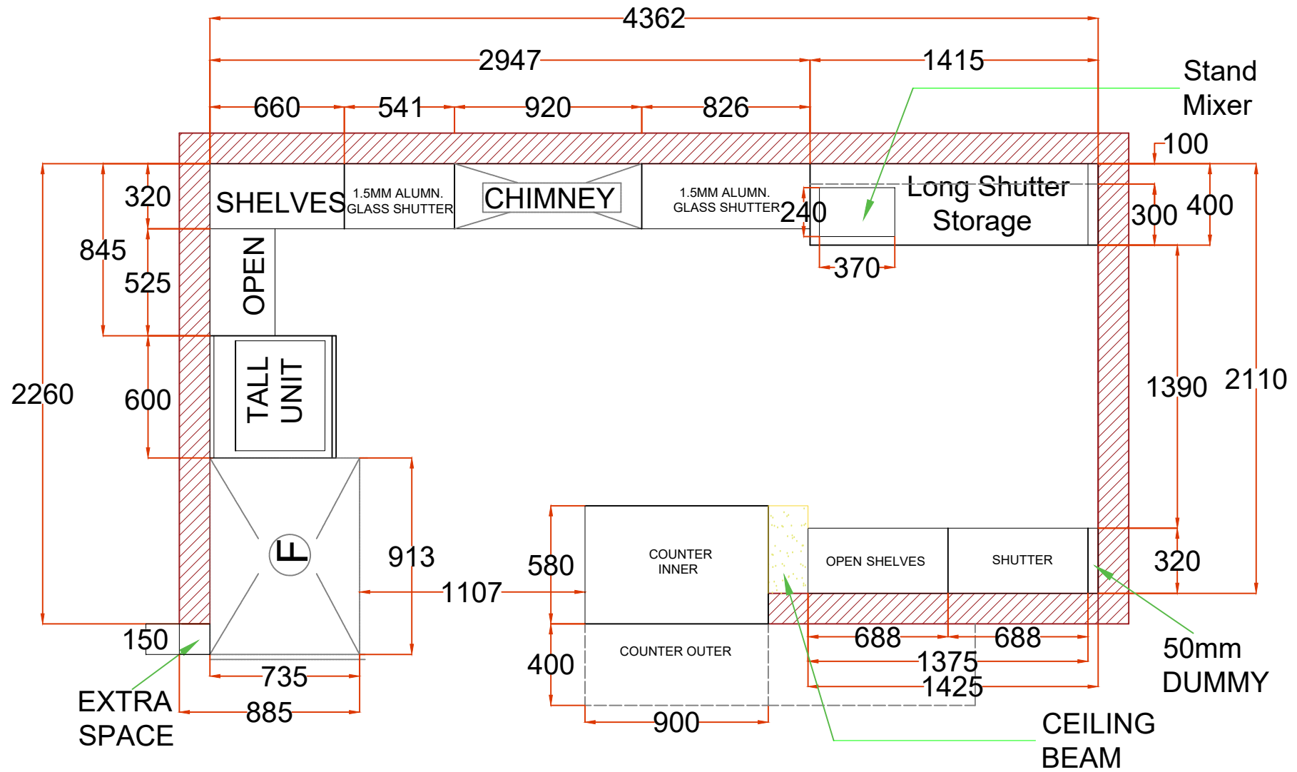
KITCHEN ABOVE UNIT PLAN
