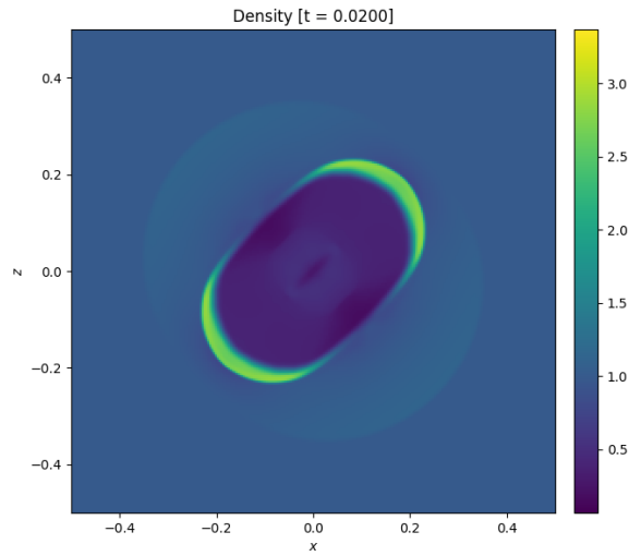
(c) 3D, Density (mid-plane slice)
