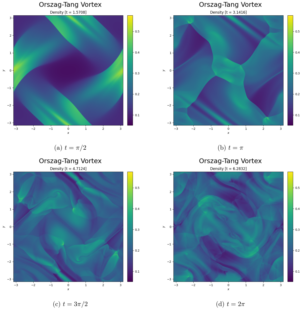
Figure 7.7: Density evolution of the Orszag–Tang vortex.
