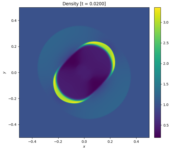
(a) 2D, Density
