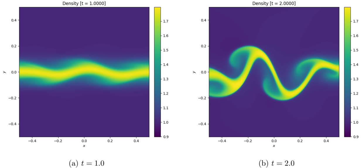
Figure 7.3: Density, showing the growth of the Kelvin–Helmholtz instability.
