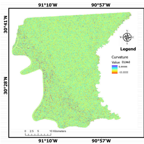
(e) Curvature
