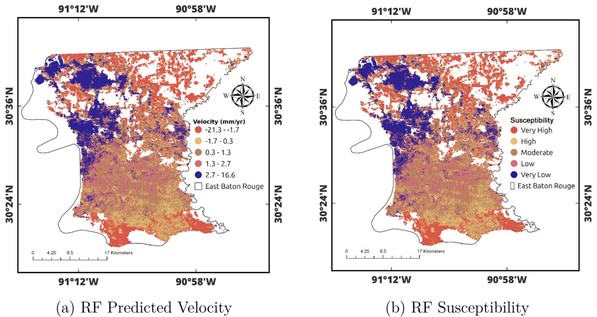
Figure 5.7. RF Model Results: (a) predicted velocity (mm/yr); (b) susceptibility classification. Spatial patterns are similar to ET but with less pronounced gradients.
