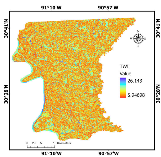
(f) TWI
