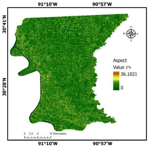
(c) Aspect
