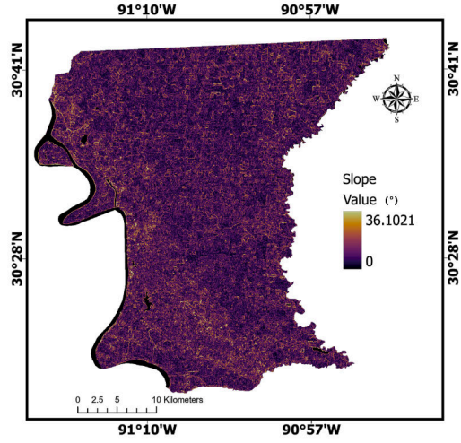
(b) Slope
