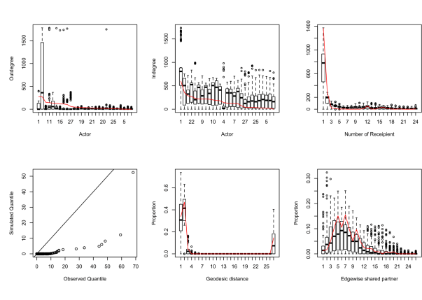
Figure 5. Posterior predictive checks for the Dare County email network: (a) outdegree, (b) indegree, (c) recipient size, (d) QQplot of time-increments, (e) geodesic distance, and (f) edgewise shared partners.
