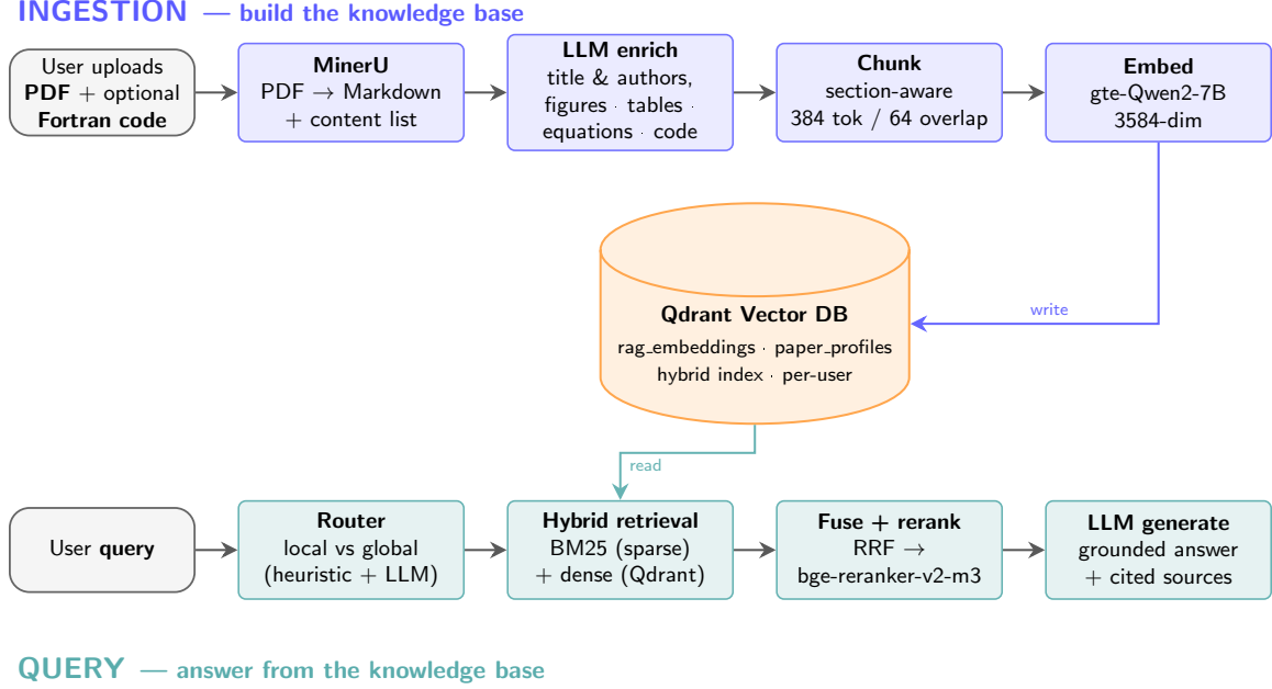
Figure 1: End-to-end RAG pipeline. Ingestion (top) writes embedded, section-aware chunks into Qdrant; querying (bottom) reads from Qdrant via hybrid retrieval, fuses and reranks candidates, then generates a grounded answer.
