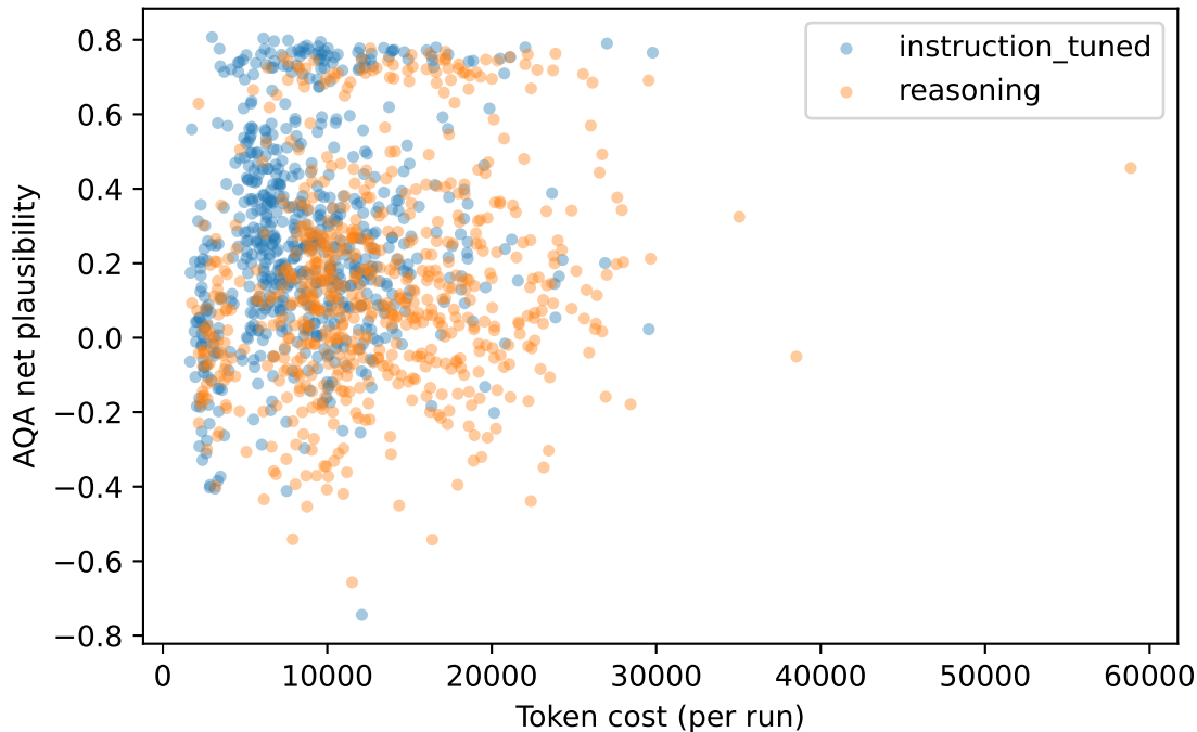
Cost vs quality
