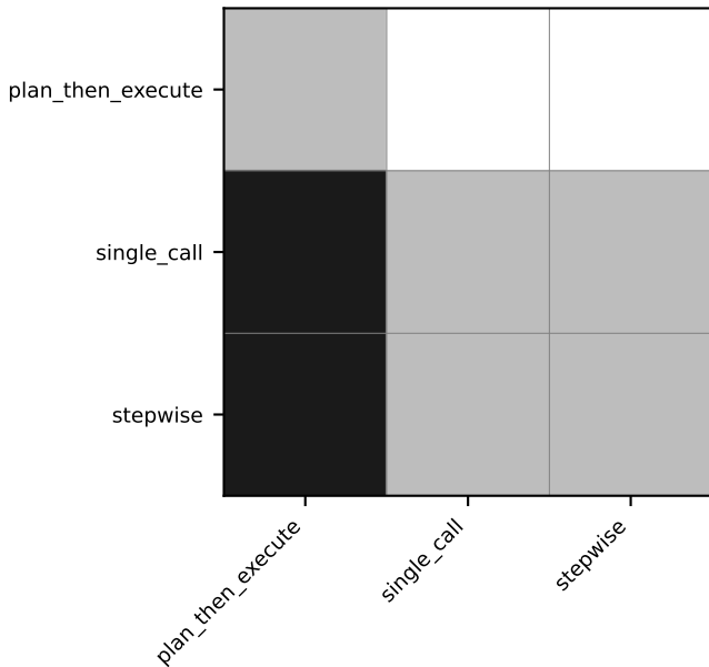
paradigm - aqa_plausibility
